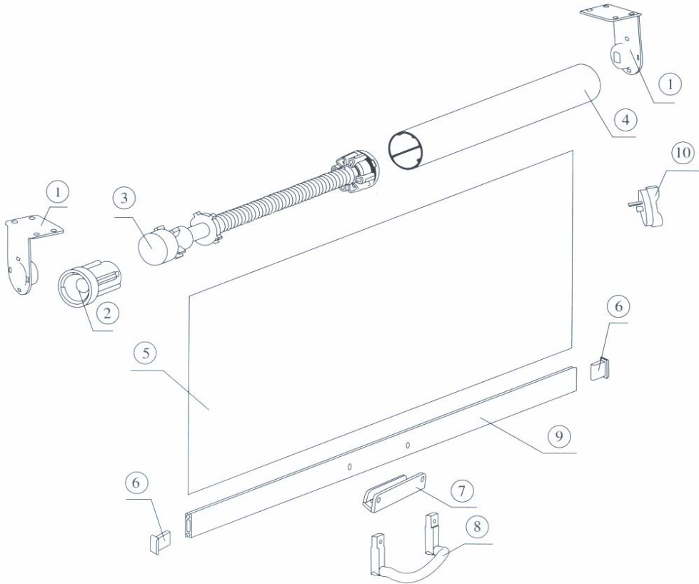
Exploded view of night blind for vertical cases
