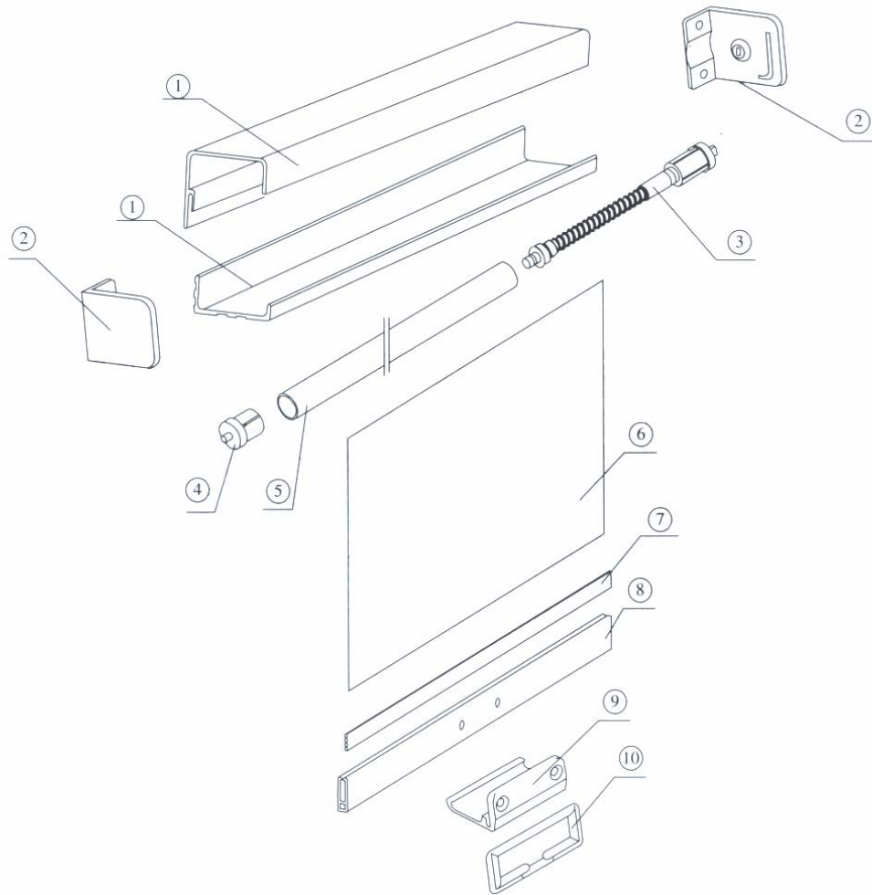
Exploded view of the Second type of night blind with aluminum cassette
