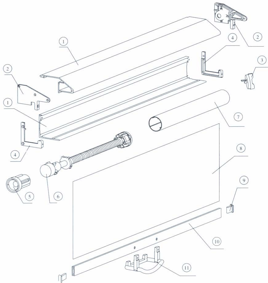
Exploded view of the first type of night blind with aluminum cassette
