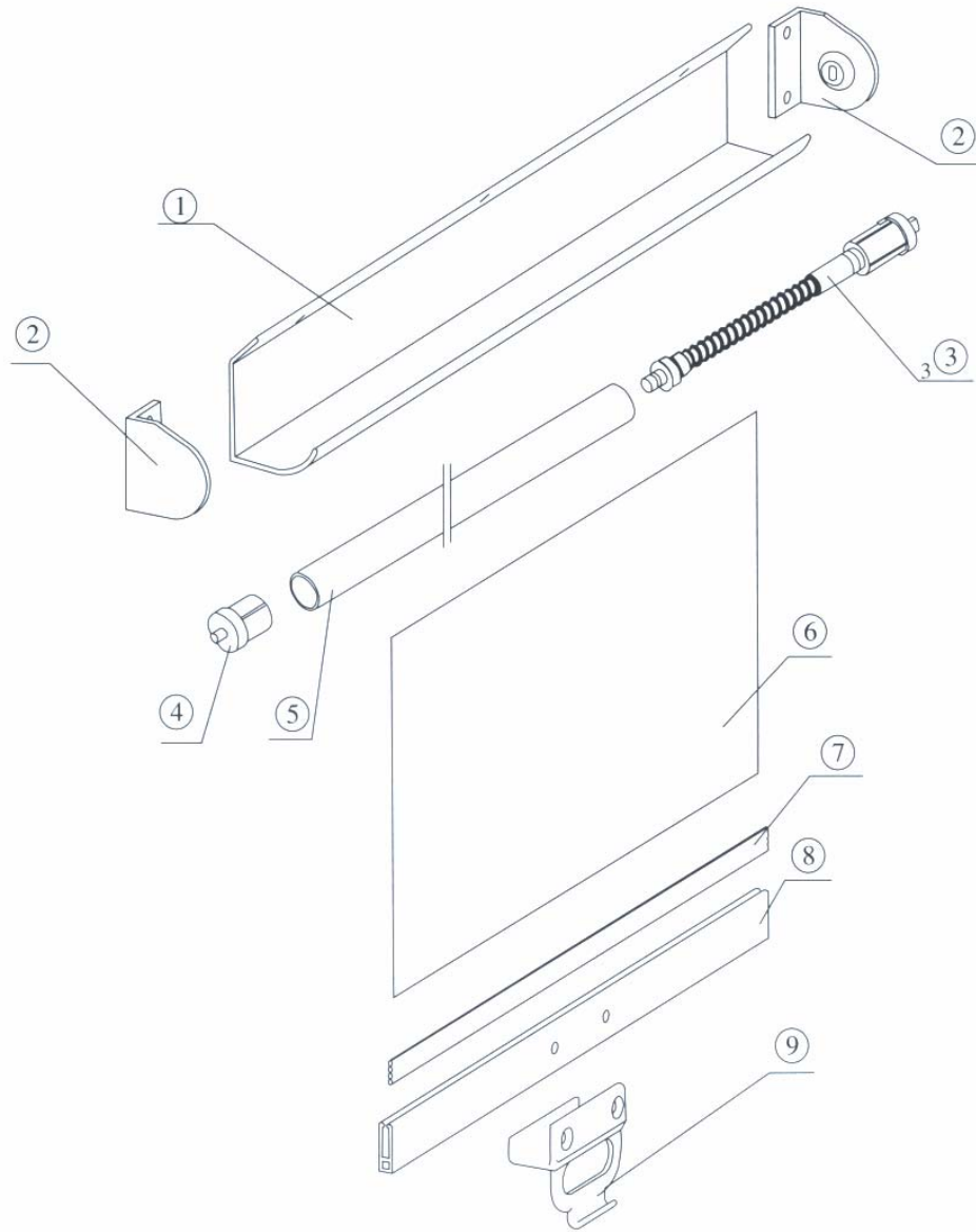
Exploded view of night blind for vertical cases
